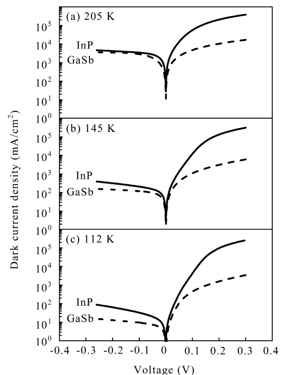
Fig. 9. Current-voltage characteristics of the sensors on InP and GaSb substrates
