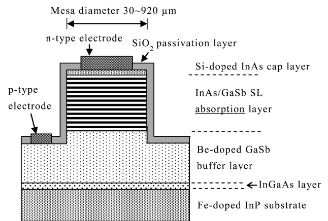
Fig. 3. Structure of the sensor on the InP substrate
