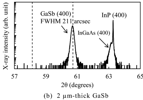
Fig. 4. XRCs of GaSb single layers on InP substrates
