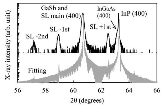
Fig. 6. XRCs of SLs grown on InP substrates
