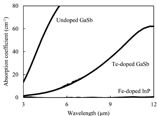
Fig. 2. Absorption coefficient spectra of InP and GaSb substrates
